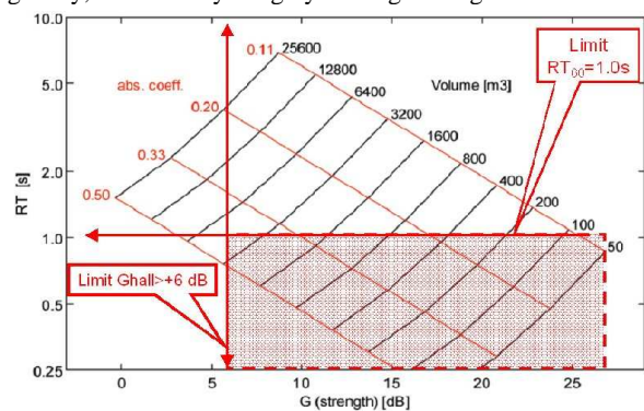
Figure 7. G-RT plot with 2 boundary-lines for theatre ( T < 1.0 s, G \geq 6 dB).
