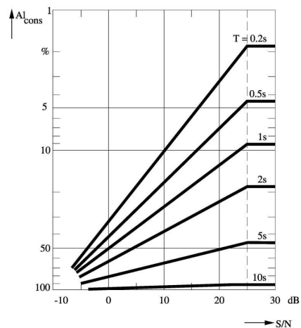
Figure 3. AL_{cons} as a function of S/N and T [1]
