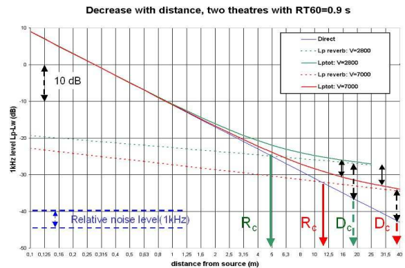
Figure 12 Decrease of sound level with distance calculated for two different theatres A (green) and B (red). The blue line gives an indication of expected noise level, assuming a average speaker as source.
