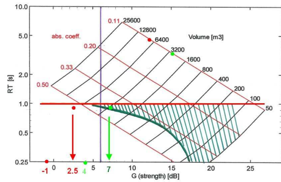
Figure 11 G-RT plot with indicated position of theatre A (green points) and theatre B (red point)
