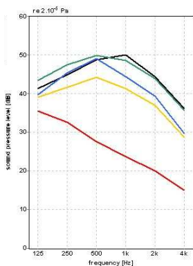
Figure 14. Measured sound level L_{eq} @row 12 during a theatre performance with non-reinforced speech in “De Spiegel” in Zwolle. Red line is background noise level, other coloured lines are several speech fragments of actors (each 2-3 minutes, 46-52 dB(A)). Red: 28 dB(A), 30 dBL, 24 PSIL. Yellow: 45 dB(A), 47 dBL. Resulting S/N=17 dB(A), 23 PSIL.
