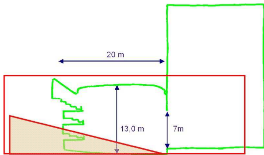
Figure 10. Schematic cross-section of theatre A (green) and theatre B (red)
