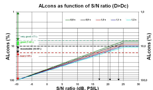
Figure 4. AL_{cons} as function of S/N for 5 values of RT.
