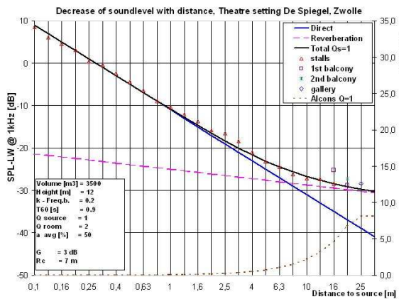
Figure 13. Decay with distance in theatre De Spiegel in Zwolle in theatre-mode, measured with an omni-directional source in the stage opening.
