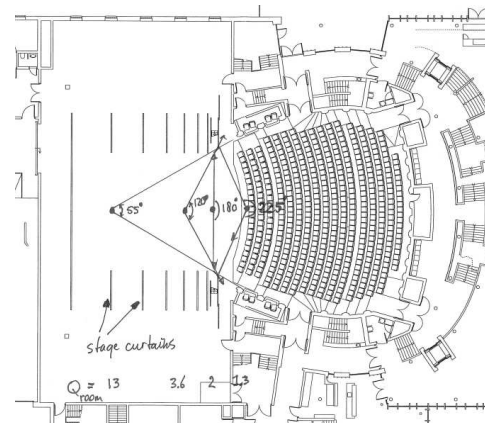
Figure 5. Ground level plan of theatre "de Spiegel" in Zwolle. For 4 different source positions, the horizontal opening angle to the hall ( \beta ) and the resulting value of Q_{room} are indicated.
