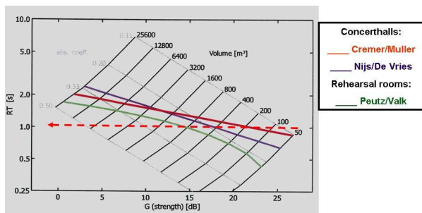
Figure 2. G-RT plot with some design lines [3,4,5]
