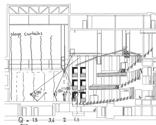
Figure 6. Cross-section of theatre "de Spiegel" in Zwolle. For 4 different source positions the vertical opening angle to the hall ( \gamma ) and the resulting value of Q_{room} are indicated.
