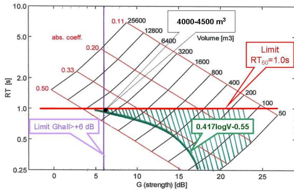
Figure 8. G-RT plot with 3 boundary lines for theatre design ( T < 1.0 s, G \geq 6 dB, eq. 16)
